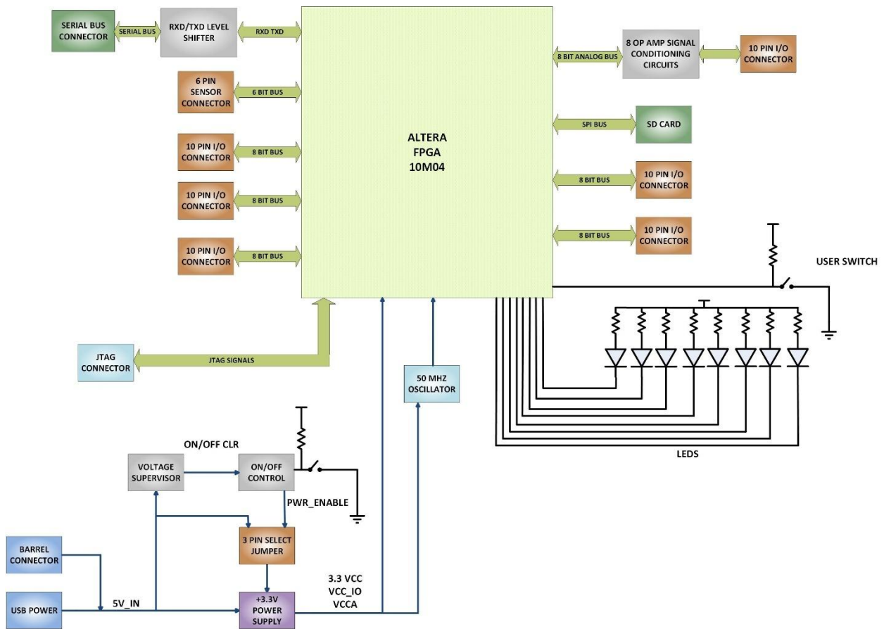
Figure 2 TRC-4CE6-AF Block Diagram
